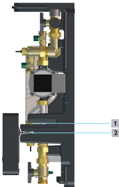
Abb. 28: Montageposition
