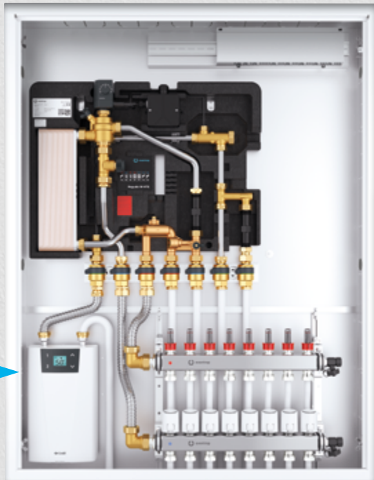
Instantaneous water heater module
