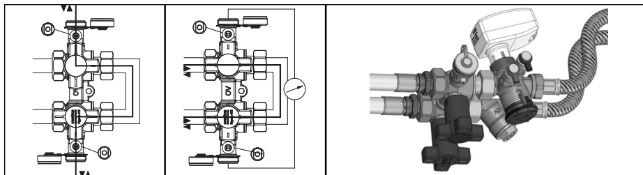
Re-filling, bleeding and flushing the appliance side (1) (2)
