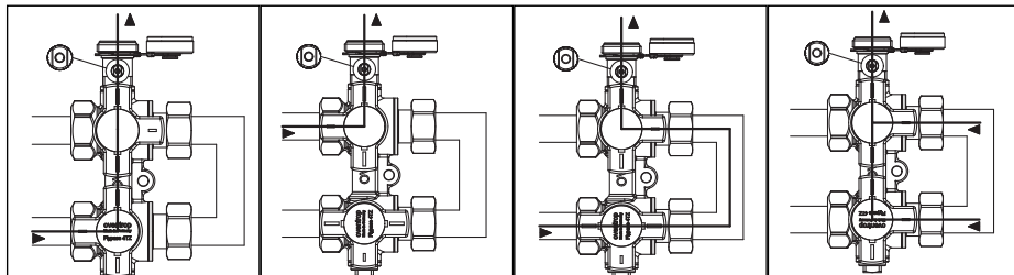
Draining of system and appliance side, bleeding and flushing the system side
