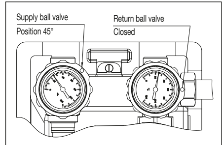
Illustr. 4.2 Filling and flushing of the solar plant
