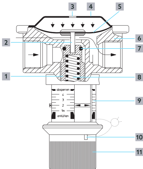
Fig. 1: Construction
