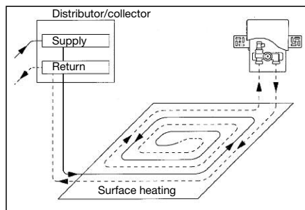
Installation sketch
