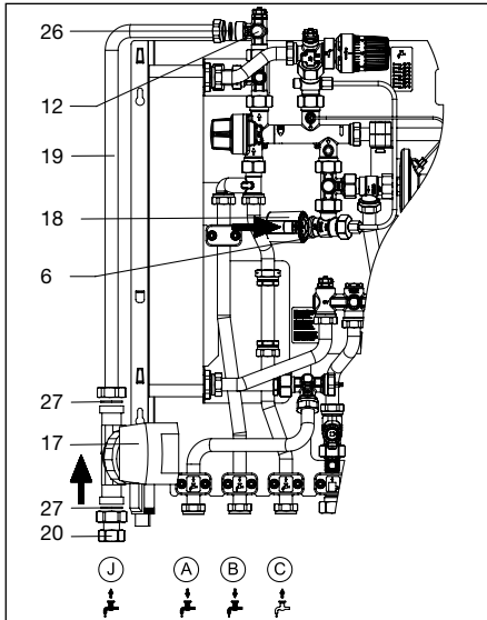
Illustr. 6.1 Installation
