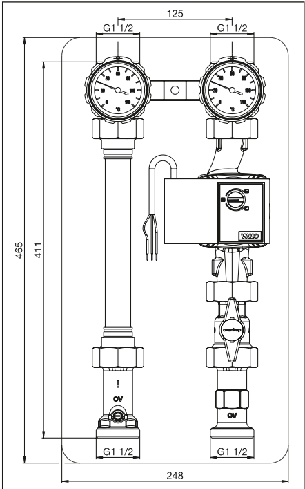
Illustr. 3 "Regumat S-180" DN 25 with pump ball valve (long version)
