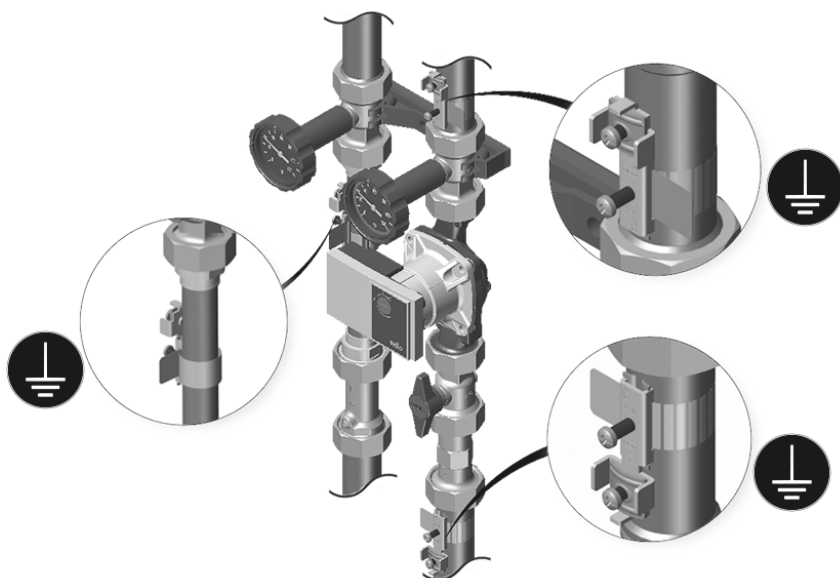
Illustr. 26 Protective equipotential bonding/grounding of an installation with metal piping
