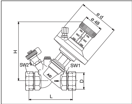
Illustr. 3: Regulator type 106 46/48 04-16 both ports male thread and collar nuts
