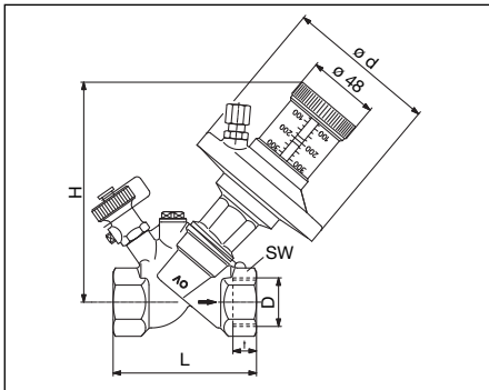
Illustr. 2: Regulator type 10645/4704-16 and 1664706-16 both ports female thread according to EN 10226
