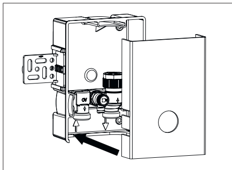
Illust. 9: Fitting of the protection cover
