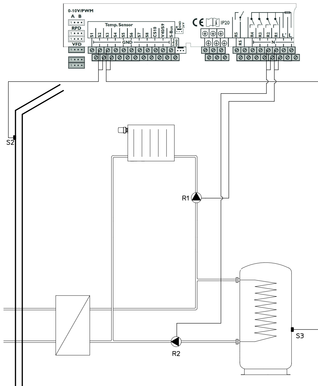
Illust. 48: Scheme 1, one constant temperature heating circuit, indirect hot potable water preparation
