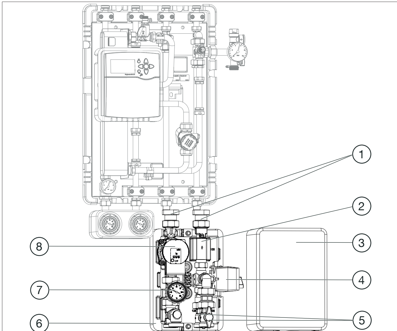
Illust. 11: Transmission station with ball valve connection set and HT switching module
