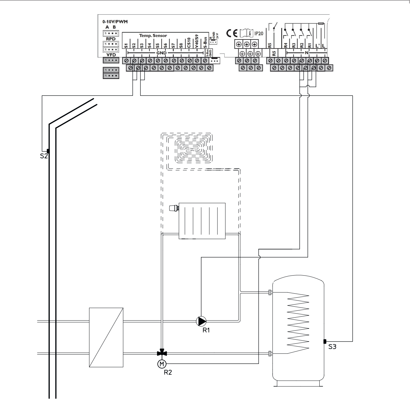
Illust. 56: Scheme 9, one constant temperature heating circuit, indirect hot potable water preparation
