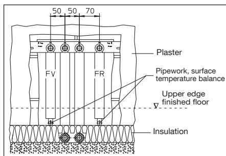
Illustr. 10 Wall view, surface temperature balance
