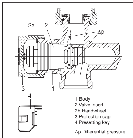
Illustr. 5 Construction thermostatic valve
