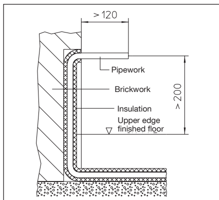
Illustr. 7 Illustrated section, heating circuit connection
