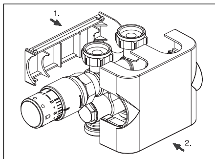
Illustr. 8 Installation of the design cover
