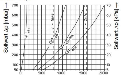
DN 50: kvs = 34,0
