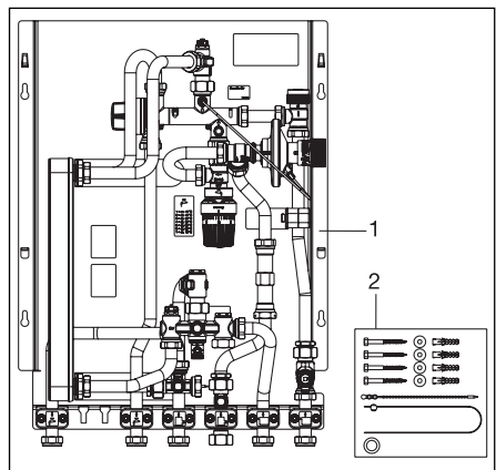
Fig. 3.1 Fourniture
