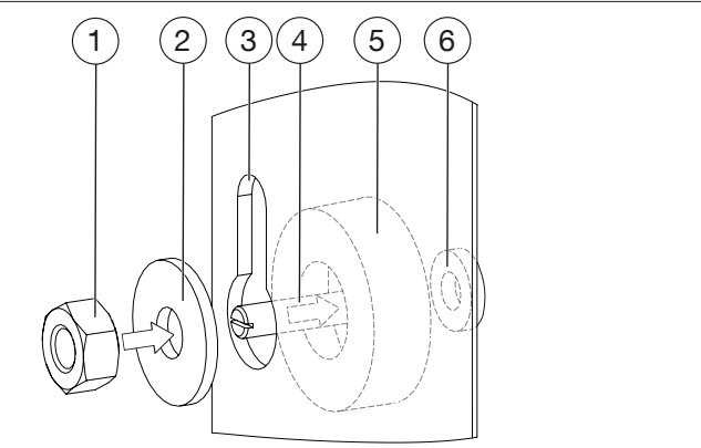
Illust. 5: Fixing points of the Regudis W-HTU
