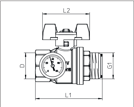
Illust. 8: Dimensions of the ball valve
