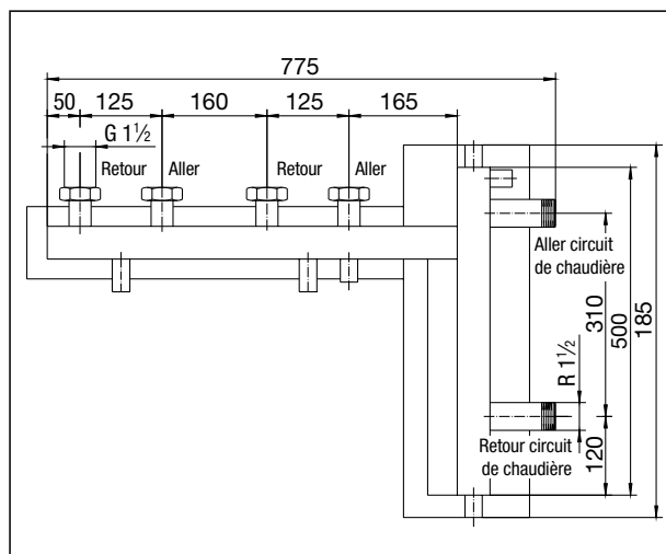
UNIT hydraulique DN 25
