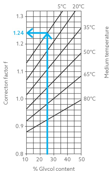
Correction factor f for propylene glycol
