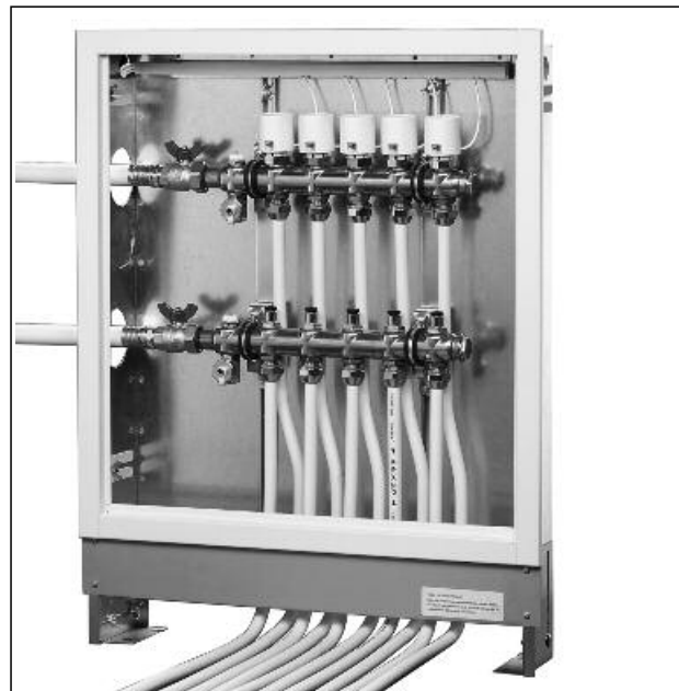
“Multidis SF” Stainless steel distributor/collector Item no. 14040..
