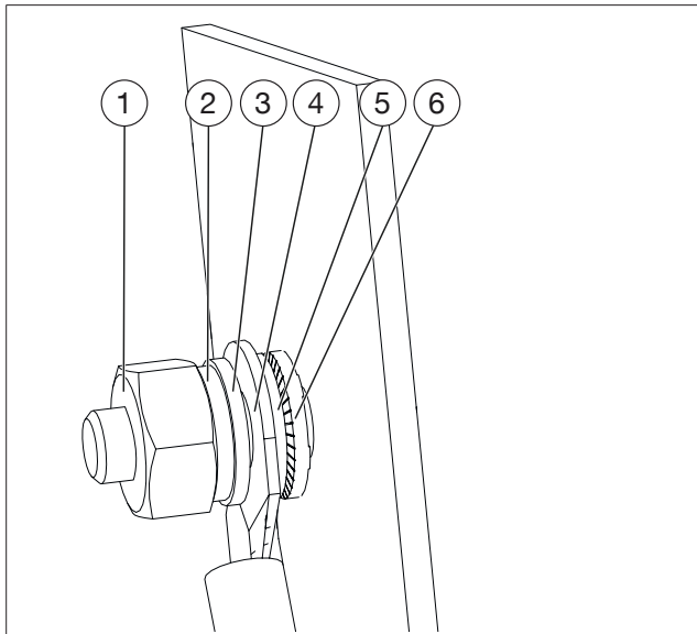
Illustr. 9: Configuration of the central earthing point
