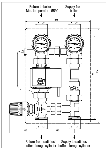
Illustr. 4.3 "Regumat RTA-130 TOP" DN25 with standard insulation Supply on right hand side Boiler is located above the "Regumat"
