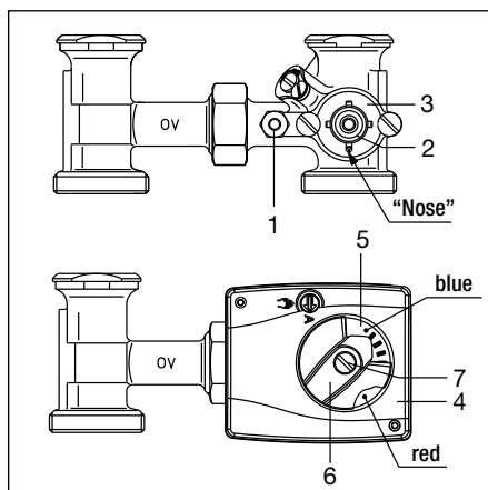
Installation three-way mixing valve
