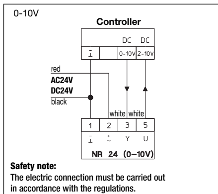
Connection diagram
