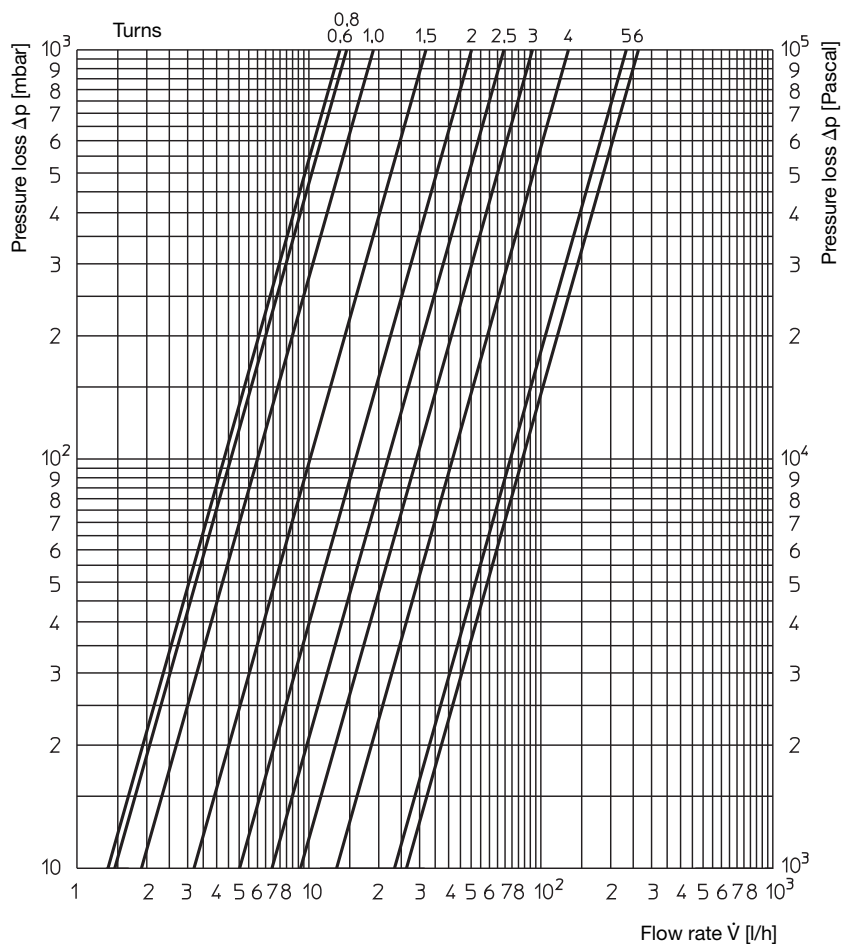
Chart 2: Pressure loss chart bypass, valve closed
