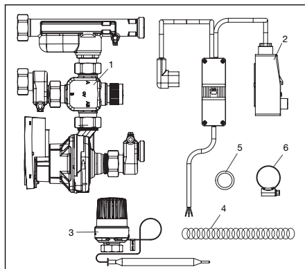
Fig. 6.1 Fourniture
