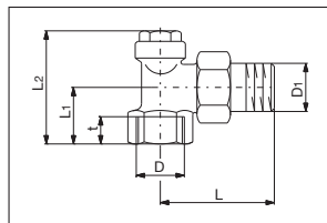
Angle pattern with female thread
