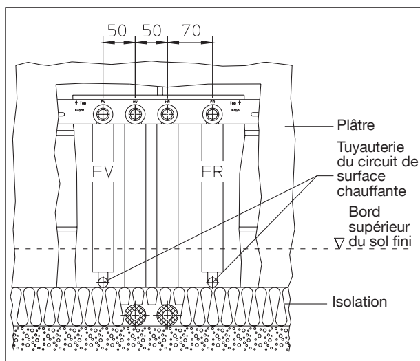
Vue frontale, raccordement circuit de surface chauffante
