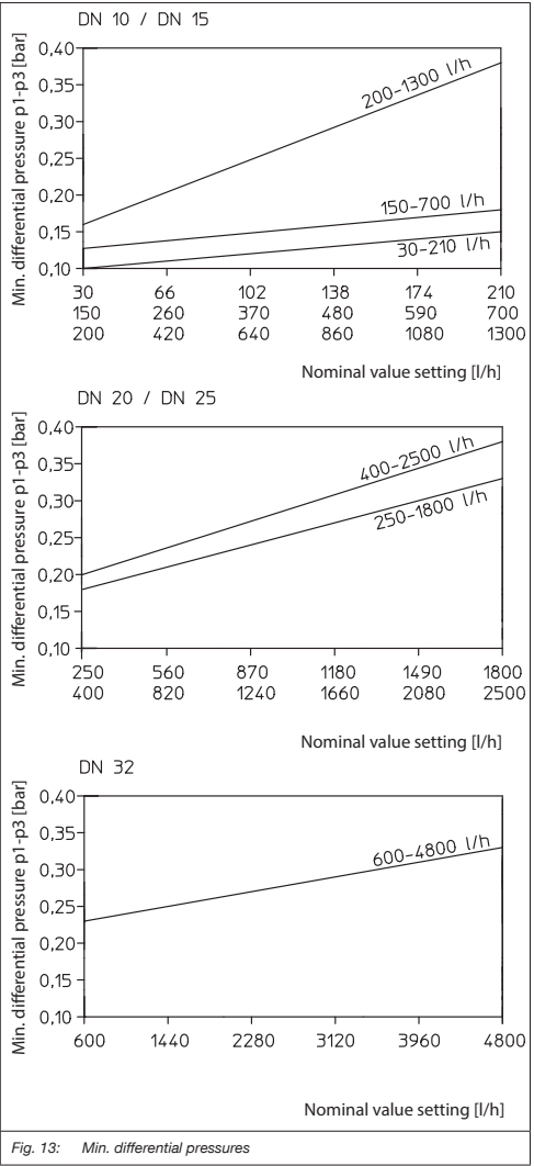
Fig. 13: Min. differential pressures
