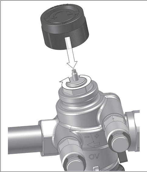
Fig. 8: Isolation
