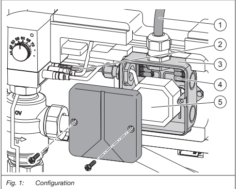
Fig. 1: Configuration
