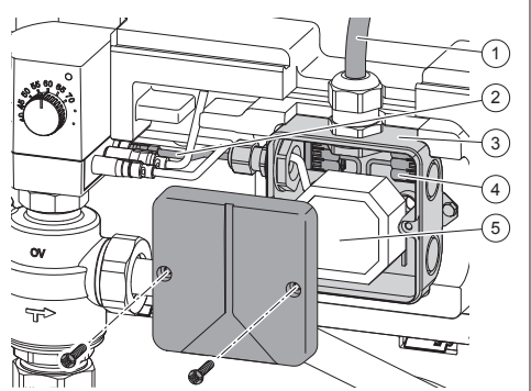
Illustr. 1: Construction
