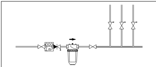
Water filter "Aquanova Compact"
