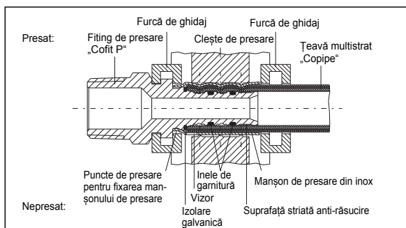
Fiting de presare Oventrop
