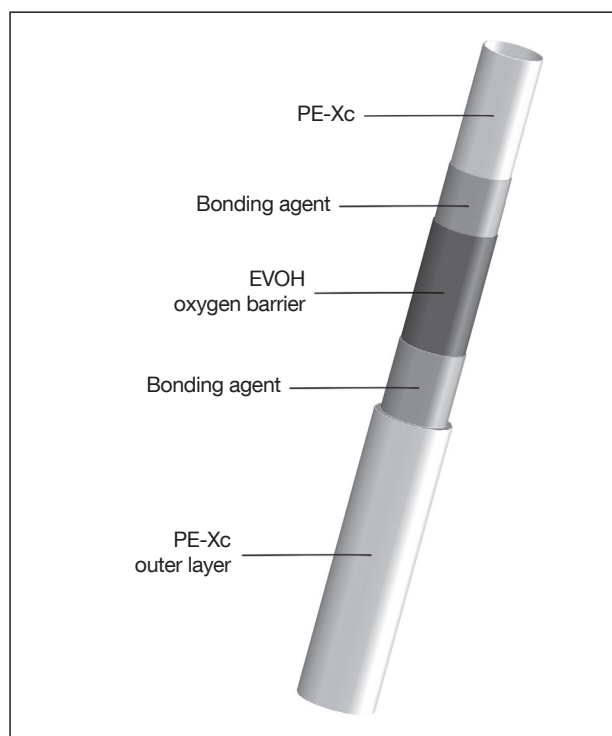
“Copex” PE-Xc plastic pipe (dimension 14 x 2 mm, 16 x 2 mm, 17 x 2 mm, 20 x 2 mm)
