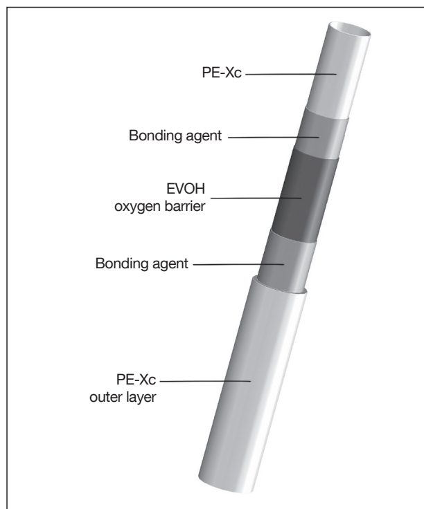
“Copex” PE-Xc plastic pipe (Dimension 20 x 2,5 mm, 26 x 3 mm, 32 x 3 mm)
