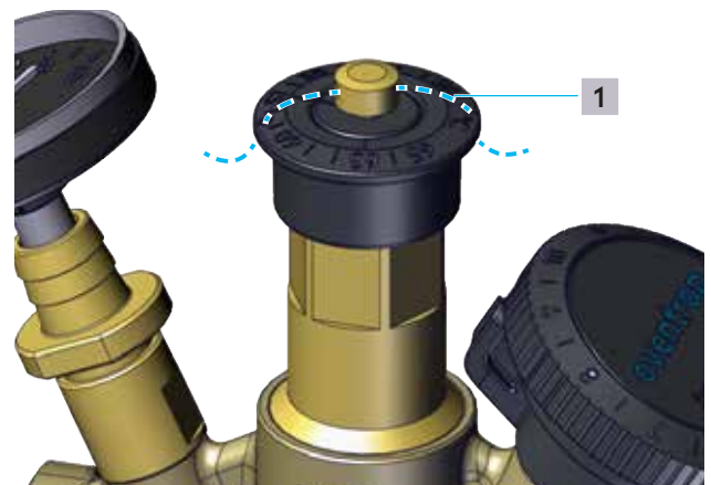
Fig. 10: Lead sealing the temperature setpoint
