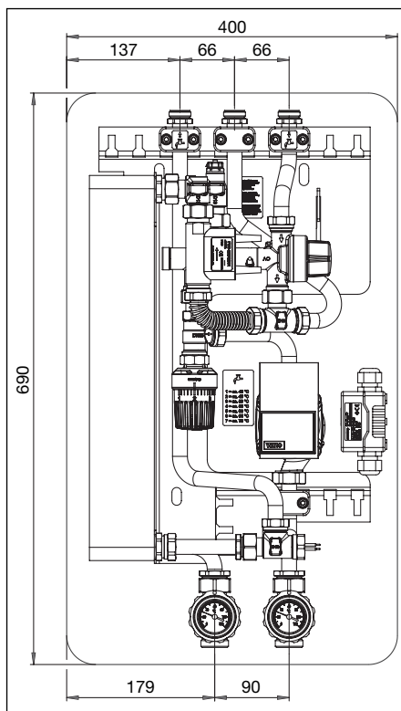
Illustr. 6.1: Installation, indications in mm
