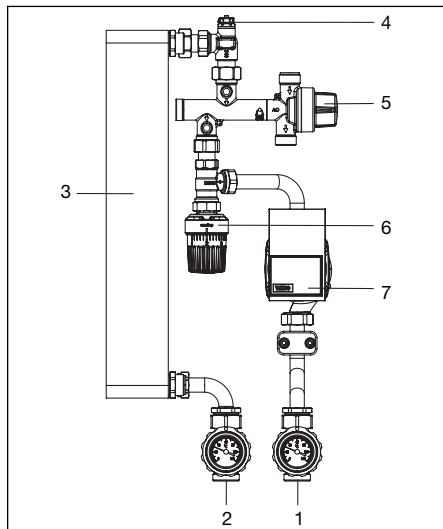
Illustr. 5.2: Primary circuit
