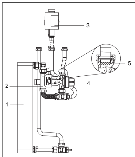
Fig. 5.3: Circuit secondaire
