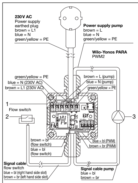
Illustr. 6.6: Cable layout primary circuit
