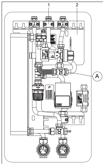
Illustr. 6.4: Connection of circulation pipes
