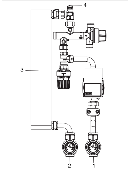
Illustr. 7.1: Bleeding "Regumaq XH"
