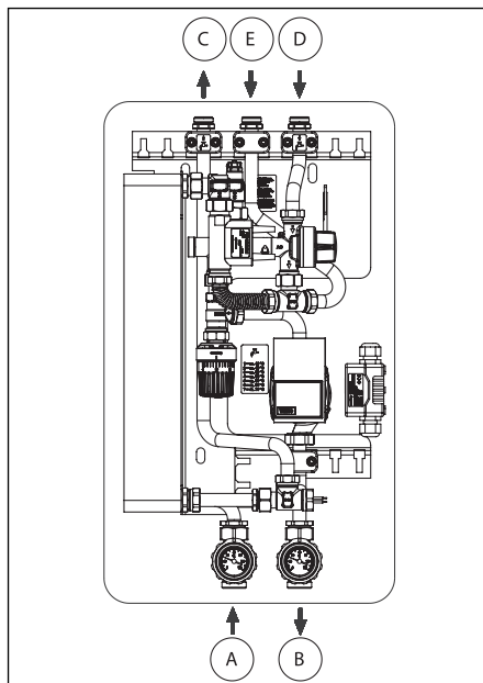
Illustr. 6.5: Connection of supply pipes
