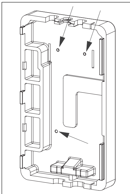
Illustr. 6.2: Rear insulation shell, drilling
