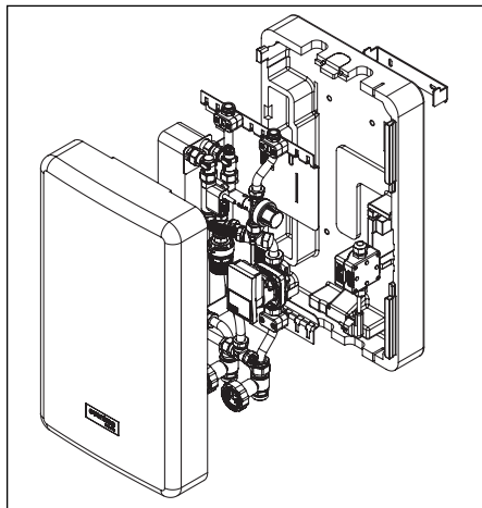
Illustr. 5.1: Overall view product assembly
