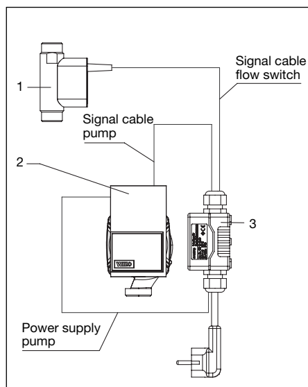
Illustr. 5.5: Electronic components
