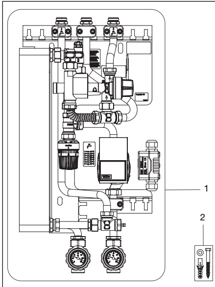
Illustr. 3.1: Extent of supply
