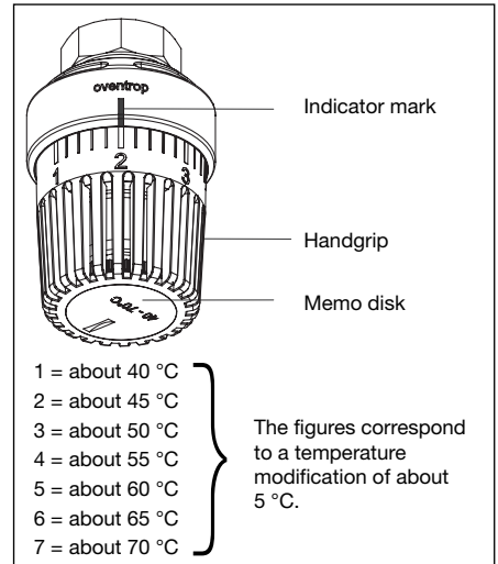
Illustr. 7.2: Temperature controller
