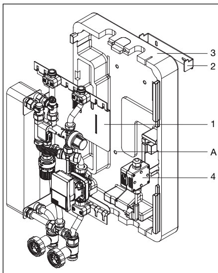
Illustr. 6.3: Wall attachment
