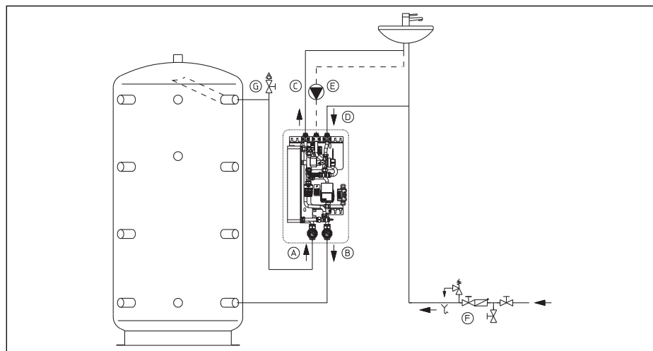
Illustr. 5.6: System illustration
