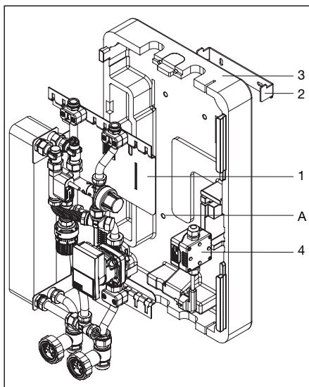
Fig. 6.3: Montage mural
