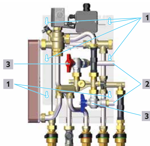
Fig. 9: Montage mural
