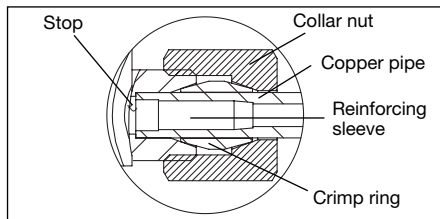
Illustr. 6.12 Illustration X, copper pipe installation
