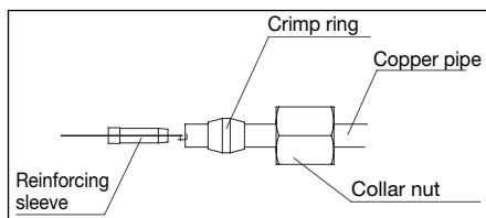
Illustr. 6.11 Installation – Part 2 1341271/1341274
