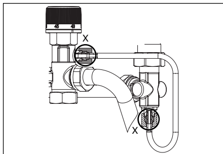
Illustr. 6.13 Installation 1341271 / 1341274
