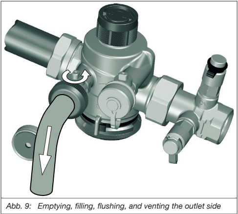
Abb. 9: Emptying, filling, flushing, and venting the outlet side
