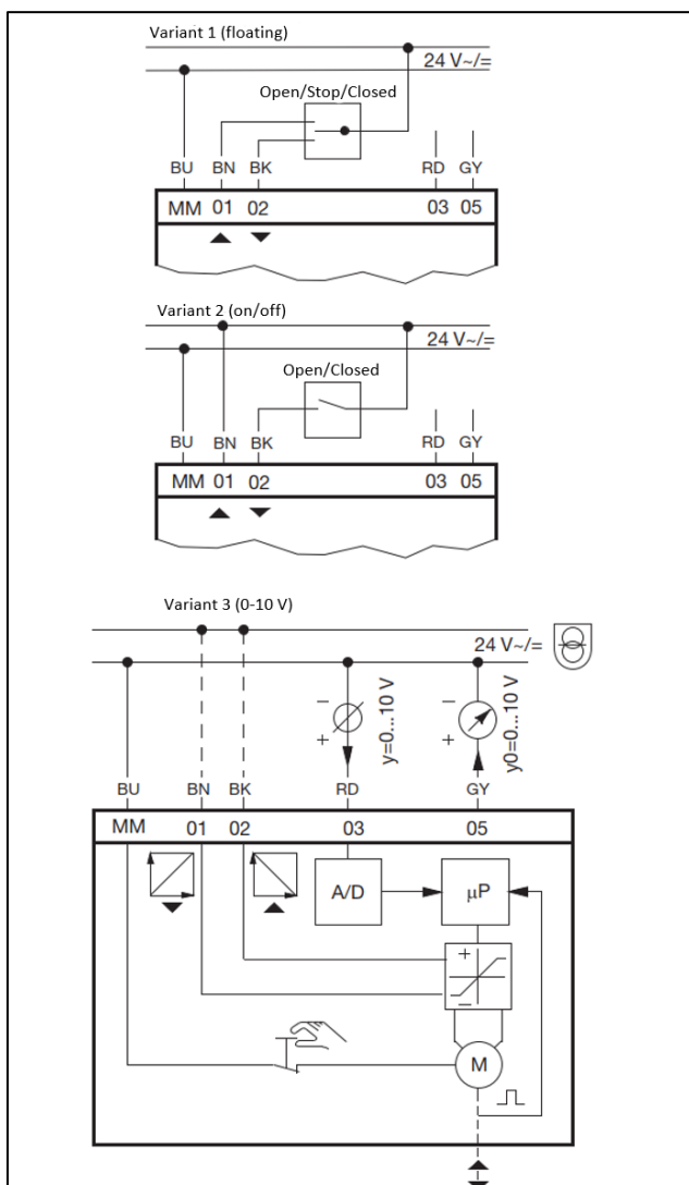
Wiring diagrams item no. 1158011
