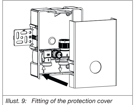
Illust. 9: Fitting of the protection cover
