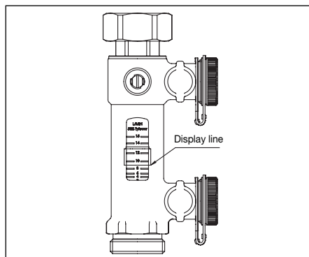
Illustr. 36 Balancing valve
