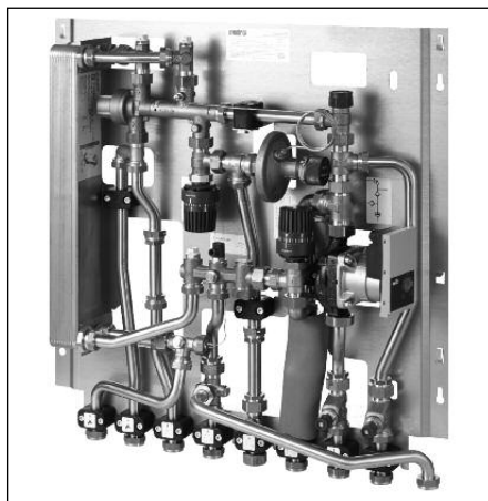
Illustr. 1.1 “Regudis W-HTF” Dwelling station with high temperature circuit
