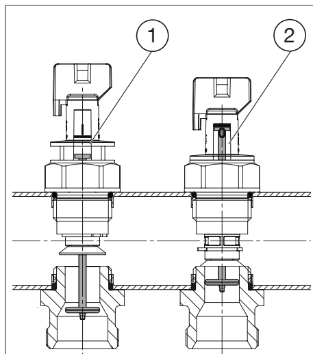
Illust. 5: Setting of the flow indicator
