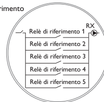
1. In parallelo (OR)
