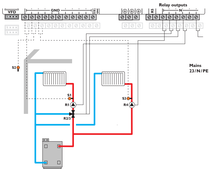
Scheme 6: 1 mixed and 1 unmixed heating circuit
