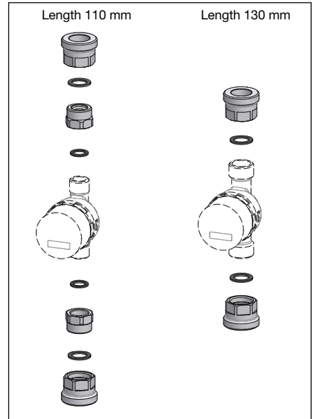
Illustr. 5.5 Installation heat meter connection set
