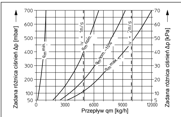
DN 40: kvs = 15,0
