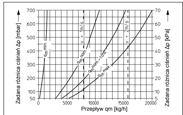
DN 50: kvs = 34,0
