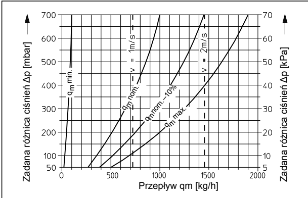
DN 25: kvs = 7,5
