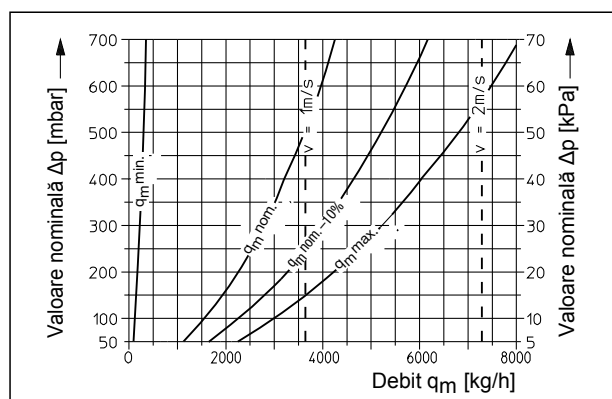
DN 32: k_{VS} = 10.0
