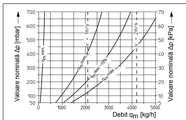
DN 25: k_{VS} = 7.5
