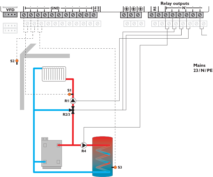
Scheme 4: 1 mixed heating circuit with DHW heating
