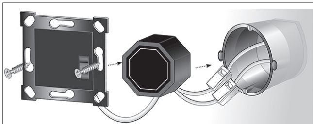
Illust. 5: Wall attachment of the fixing plate and flush-mounted power pack
